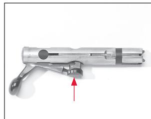
The bolt handle must be in the unlocked position prior to installation.
