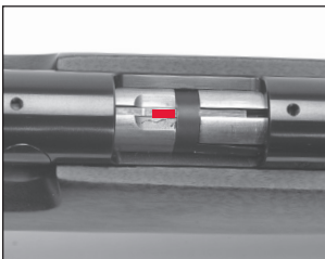
The cocking indicator showing the firing pin is in the cocked position.
